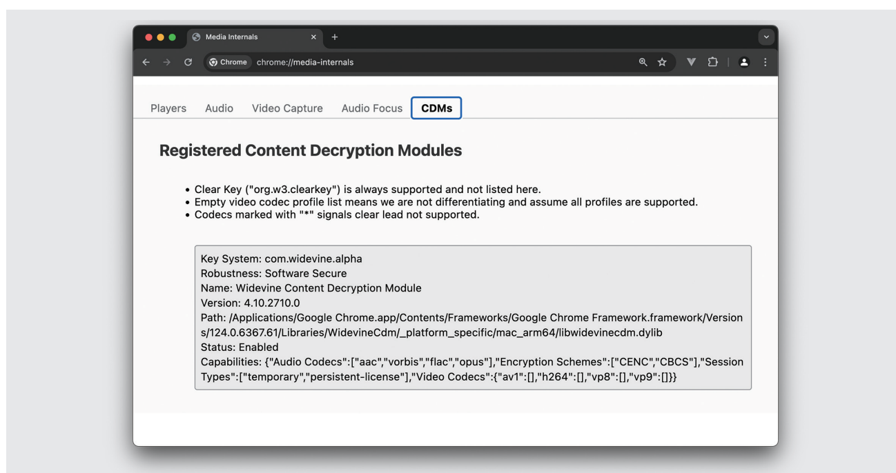
図-2 Chromeのmedia-internals
